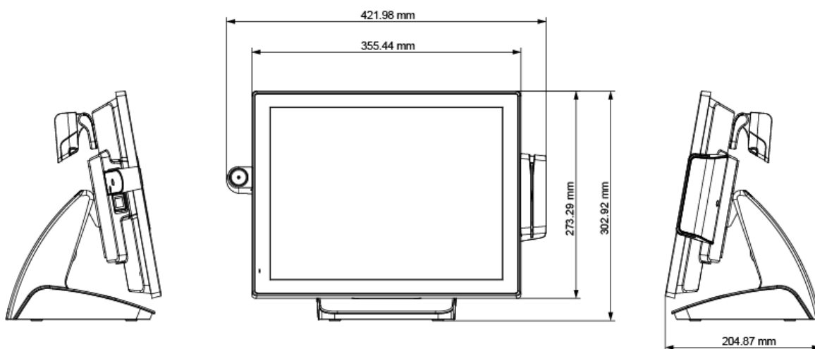
Left View
